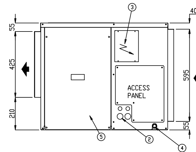
R/H ELEVATION
